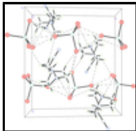
Fig. 2. Crystal structure of the title compound with view along the a axis. Intermolecular interactions are shown as dashed lines.
